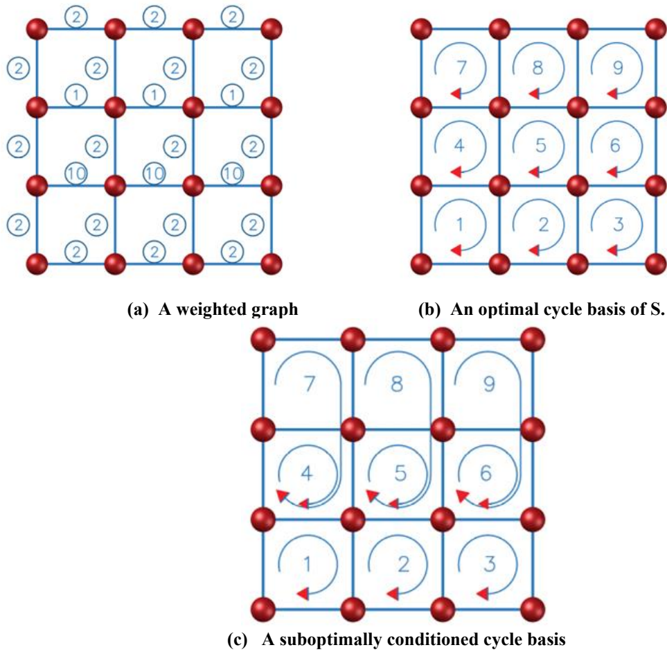
Figure 16: A single-layer rigid-jointed grid S.
