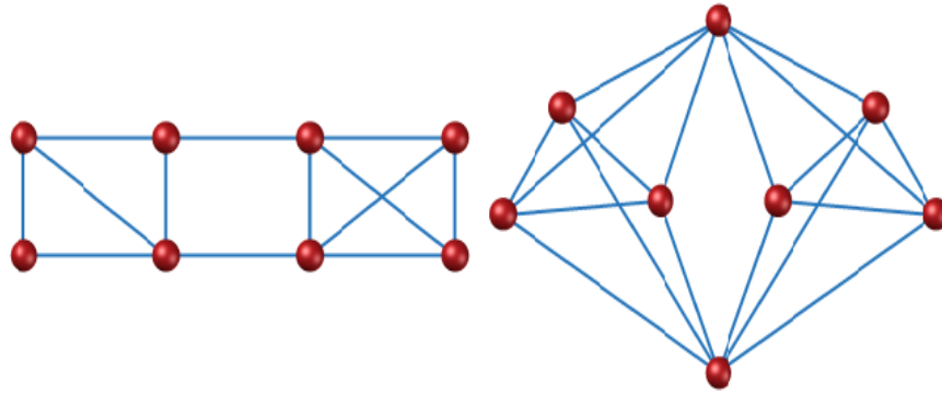
(a) \gamma(S)=M-2N+3 . (b) \gamma(S)=M-3N+6 . Figure 7: Structures satisfying \gamma(T) = 0 which are not rigid.
