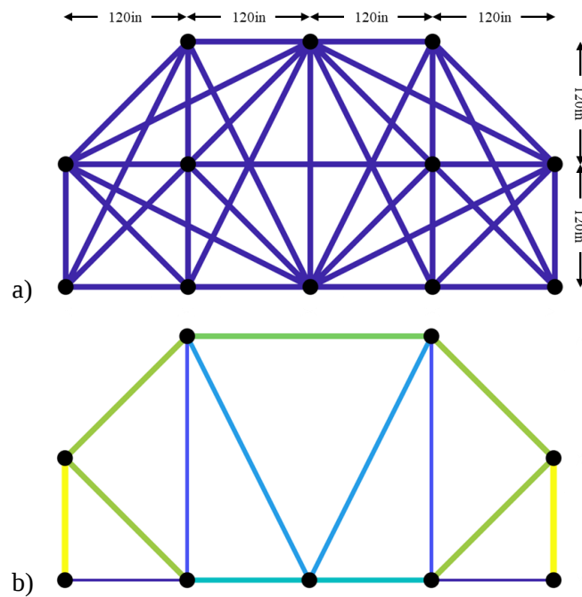
Figure 6: Comparison of the initial ground structure (a) and optimized size and topology (b) for a 39-Bar Truss Structure
