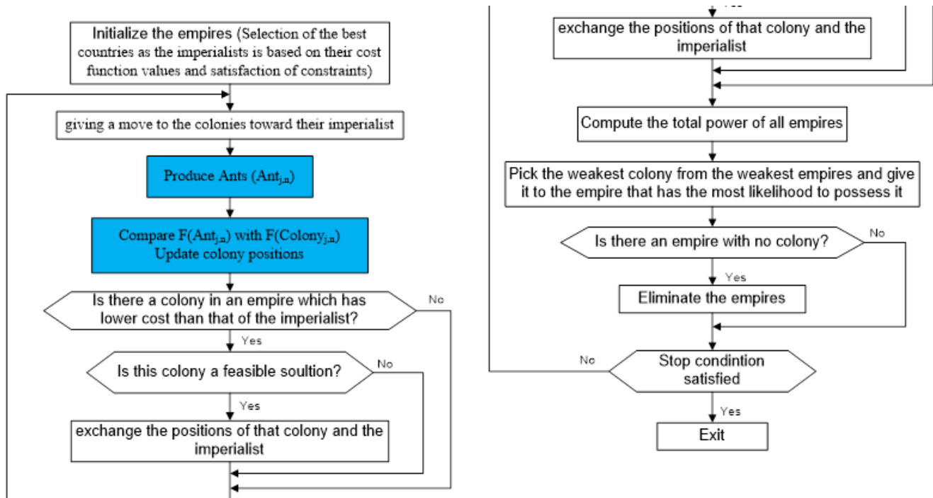
Figure 6. Flowchart of the imperialist competitive ant colony optimization [11]
