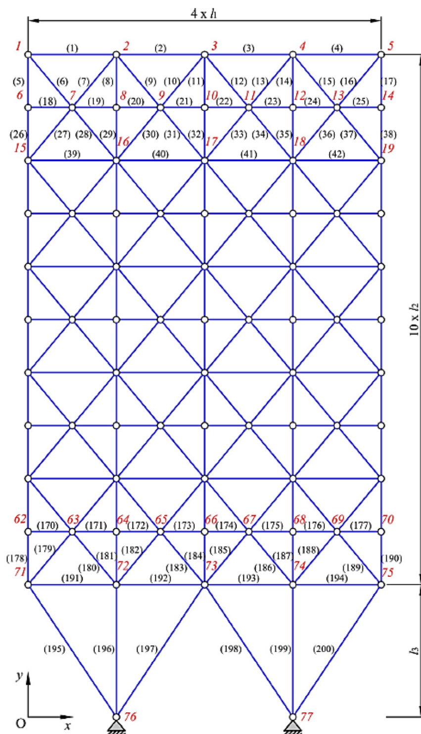
Figure 6. 200-bar truss
