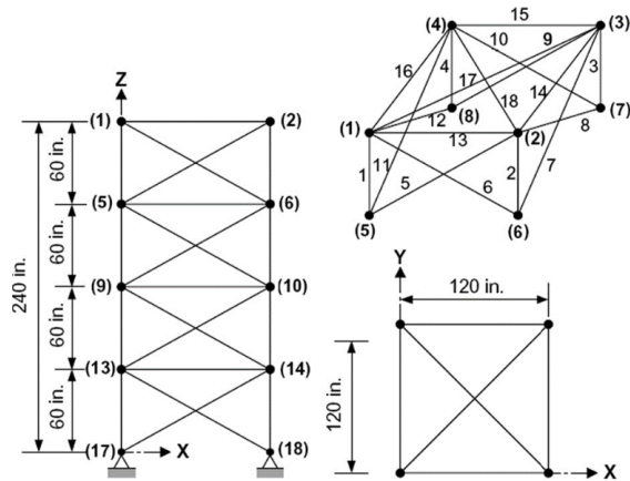
Figure 9. Seventy two-bar spatial truss
