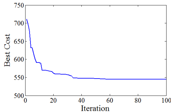
Figure 8. Convergence history for the optimum solution of the twenty five-bar spatial truss
