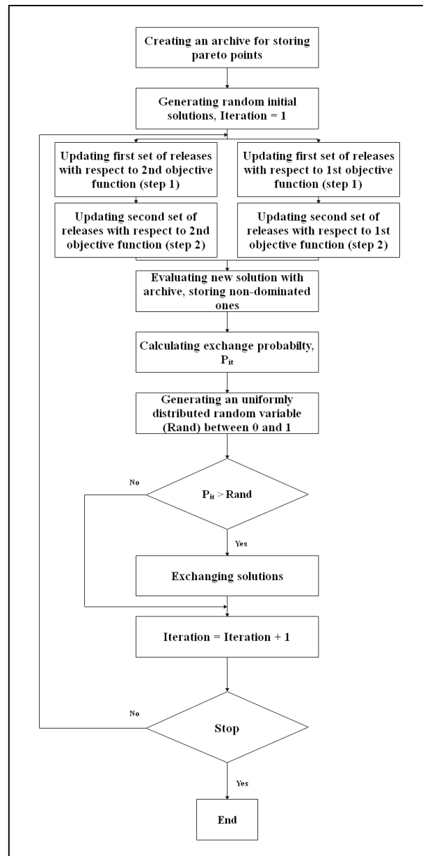
Figure 2. A 2-Step Parallel Cellular Automata flowchart for reservoir operation optimization
