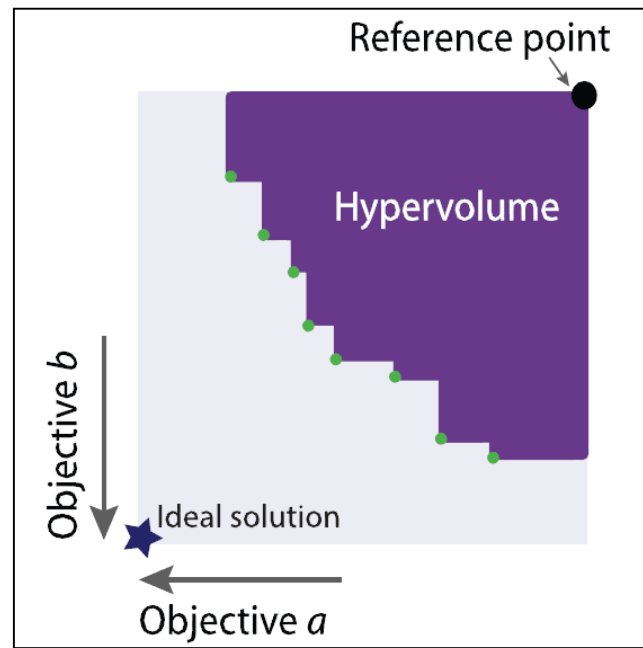
Figure 1. Hypervolume illustration
