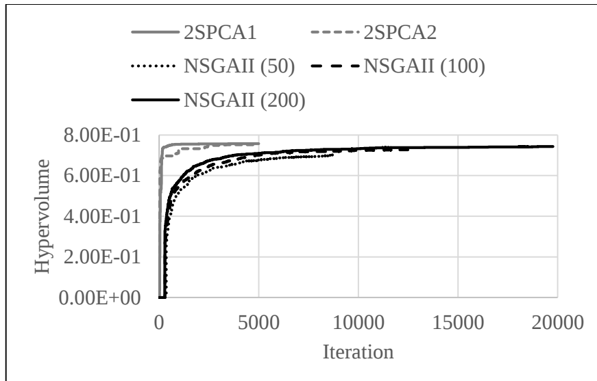
Figure 8. Hypervolume value versus iteration number
