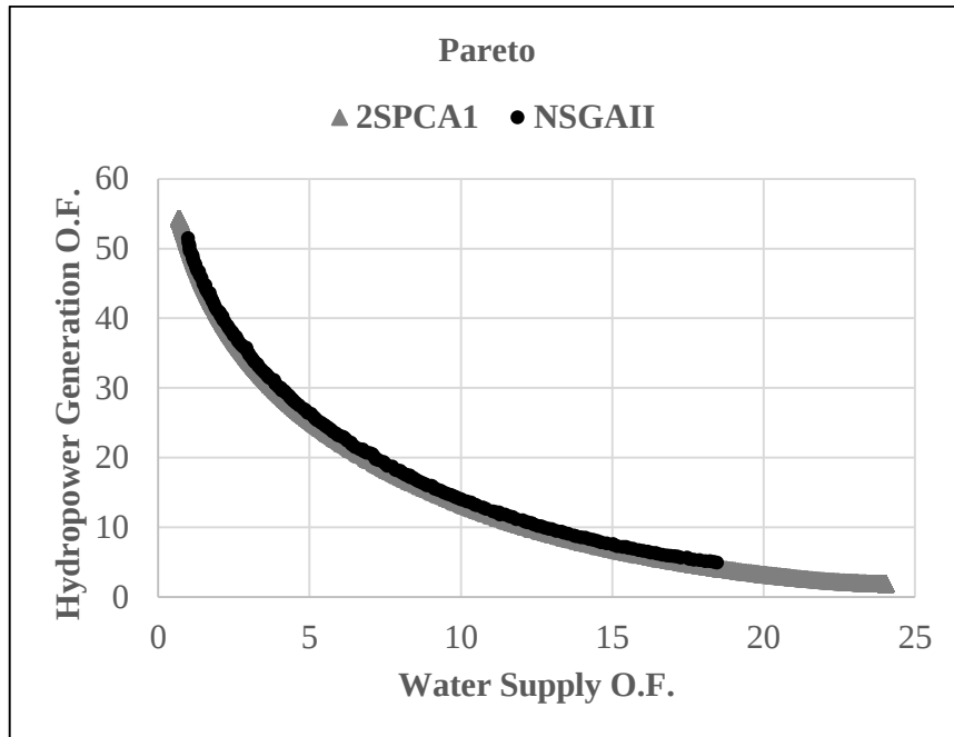
Figure 7. 2SPCA1 and NSGAII (population size of 200) paretos
