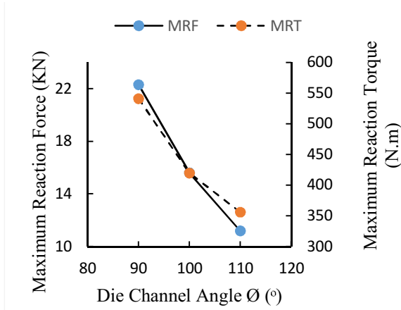
Fig. 6. Comparing the forces and torques acting on the axis of rotation for angles of 90°, 100° and 110°.
