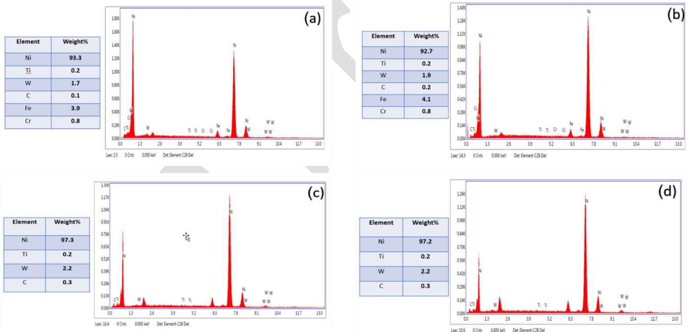
Fig. 3: EDS analysis of Ni–WC–TiC composite coating at different current densities: a) 30 mA/cm², b) 35 mA/cm², c) 40 mA/cm², and d) 50 mA/cm²
