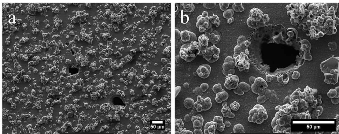
Fig. 9: SEM images of the surface of the coated sample with a current density of 40 mA/cm 2 after corrosion in 3.5 wt.% NaCl solution with two different magnifications
