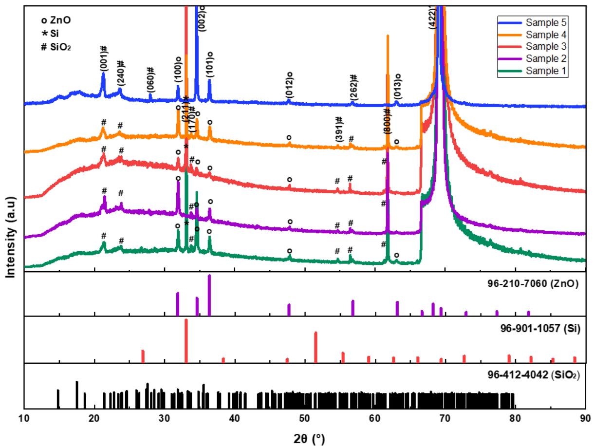
Fig. 4. XRD spectrum of the ZnO rods grown on P5Si
