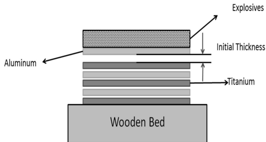
Fig. 1. Schematic presentation of parallel setup used for Ti-Al multilayer explosive welding.
