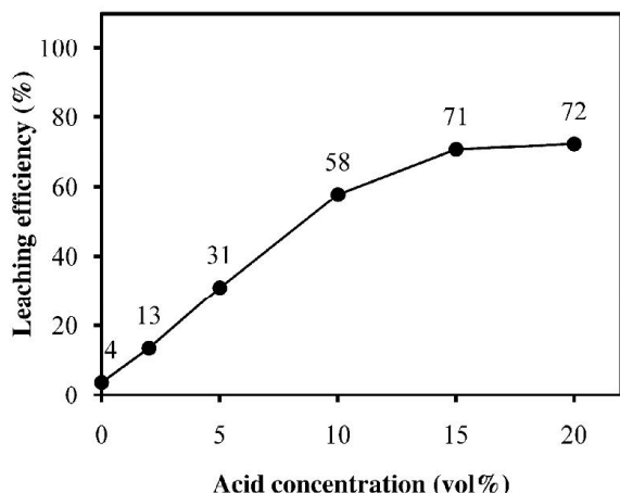
Fig. 1. Effect of acid concentration on the vanadium leaching efficiency. Other constant parameters are: temperature: 60 °C, acid/TPPA ratio: 10, leaching time: 120 minutes and particle size of 75 - 150 \mu\text{m} .
