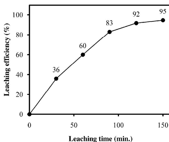
Fig. 4. Effect of leaching time on the vanadium leaching efficiency. Other constant parameters are: acid concentration: 15%, temperature: 75 °C, acid/TPPA ratio: 15 and particle size of 75 - 150 \mu\text{m} .
