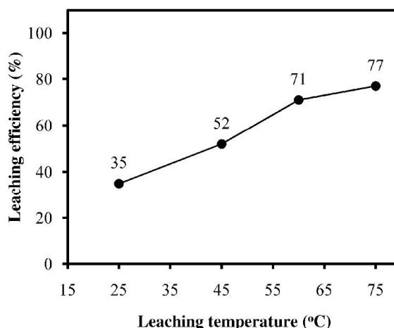
Fig. 2. Effect of leaching temperature on the vanadium leaching efficiency. Other constant parameters are: acid concentration: 15%, acid/TPPA ratio: 10, leaching time: 120 minutes and particle size of 75 - 150 \mu\text{m} .
