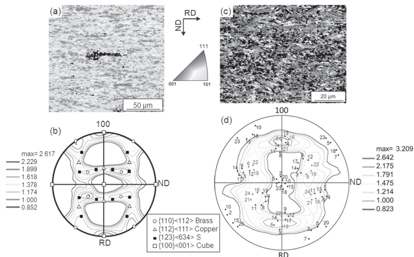
Fig. 6. EBSD orientation color maps and \{100\}_A pole figures of austenite after 6 cycles of ARB process ((a), (b)) EBSD orientation color maps and \{100\}_M pole figures of martensite transformed from the 6-cycle ARB processed specimen having elongated ultrafine-grained austenite ((c), (d)). The positions of the ideal \langle 100 \rangle_M axes for the 24 variants of martensite transformed from the austenite with exact Brass orientation ( (011) [2 \bar{1} 1]_A ) from the austenite are shown by the numbers in \{100\}_M pole figure of (d). The preferential variants are indicated by red color.
