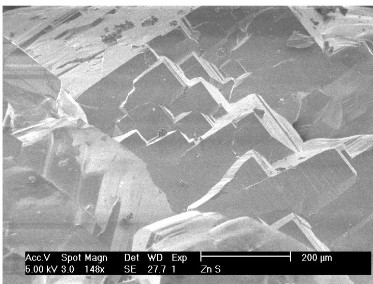
Fig. 10. Kinks formed on rough surface of ZnS crystals grown at 1102 °C
