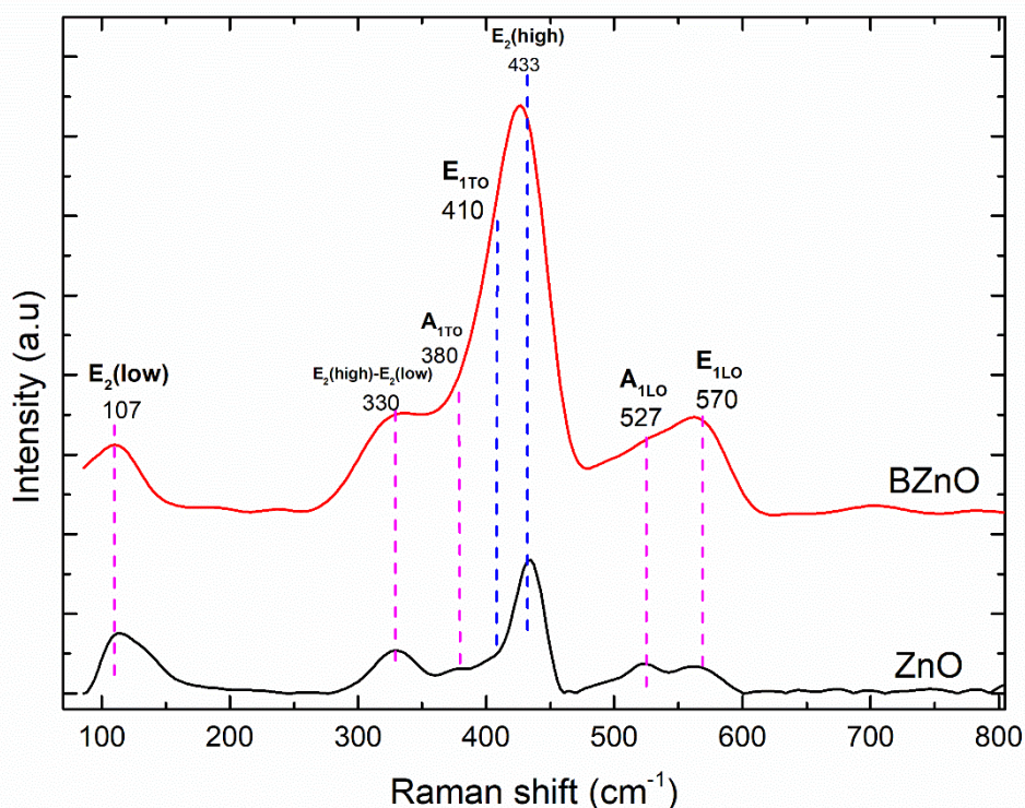
Fig.5 shows the Raman spectra of the BZnO and ZnO microrods recorded at room temperature in the range of 90–800 \text{cm}^{-1} . As shown in Fig.5, the most intense Raman peak at 433 \text{cm}^{-1} was one of the characteristic peaks of wurtzite ZnO which corresponds to the 1 st order non-polar active Raman mode of ZnO E_2 (high) associated with the vibration of O atoms in the ZnO lattice. The observed peaks at 107, 330, 380, 410, 525 and 570 \text{cm}^{-1} are the phonon modes E_2 (low), E_2 (high) - E_2 (low), A_1 (TO), E_1 (TO), A_1 (LO) and E_1 (LO) [31, 32]. The 2 nd order mode of E_2 (high) - E_2 (low) is due to interstitial defects in the atomic structure of ZnO. The appearance and position of these peaks confirm that the grown structures were wurtzite ZnO with high crystal quality [33]. In agreement with the XRD results, the Raman spectra show peaks corresponding to the phonon modes of hexagonal wurtzite ZnO. Fig.5 also shows that the BZnO spectrum exhibits an increase in peak intensities as well as overall broadening for all vibrationa modes in the 90–800 \text{cm}^{-1} range, particularly for the E_1 (LO) and E_2 (high) modes. The peak at 570 \text{cm}^{-1} is assigned to the E_1 (LO) mode and is due to impurities and structural defects such as oxygen vacancies V_O and Zn interstitials Zn [34, 35]. This observation is explained by an increase in the concentration of intrinsic defects in the branched microrods. This observation is consistent with the work of Liu et al. on ZnO nanorods after branching, where a similar increase in the intensity of the E_1 (LO) mode was also observed [36]. Raman spectroscopy analysis revealed a significant increase in the intensity of the E_2 (high) mode and
