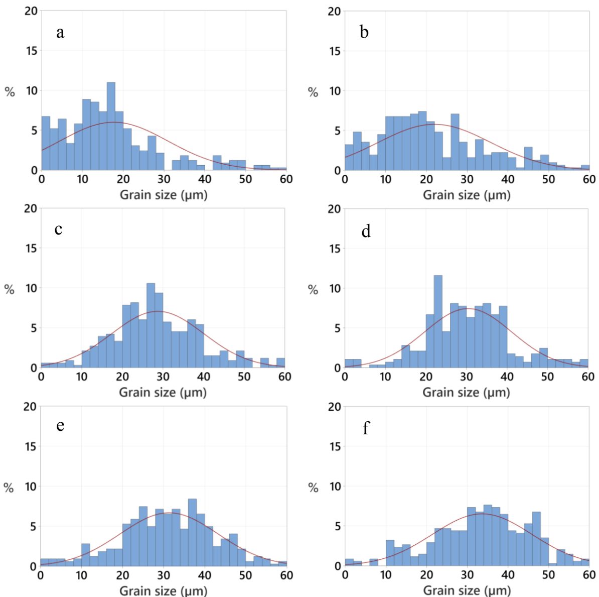
Fig. 13. Grain size distribution of hot compression samples, at (a, b) 950°C, (c, d) 1050°C, and (e, f) 1150°C, and strain rates 1 and 0.1 s -1 respectively
