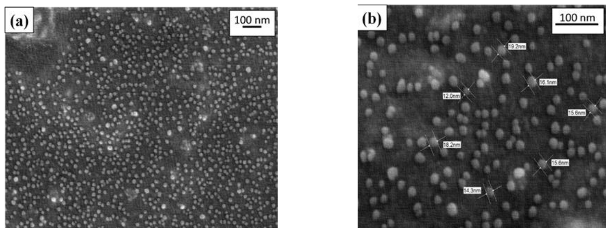
Fig. 4. FESEM image of EBN-AgNPs in 80\times (a) and 200\times (b).
