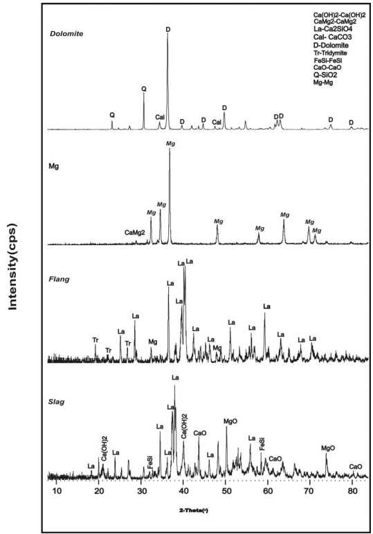
Fig. 4. XRD pattern of Asian Abe-Garm dolomite, Mg crown, white precipitated inside flange and slag.
