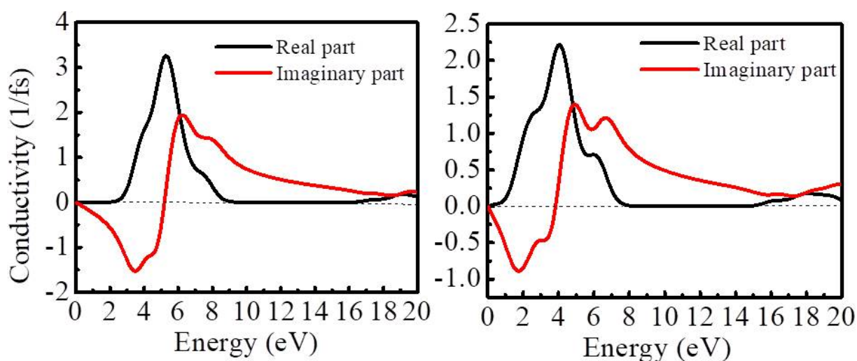
(a) \text{SrTi}_{0.875}\text{Cr}_{0.125}\text{O}_3
