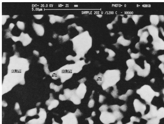
Fig.1. SEM micrograph of the starting clinker containing 40wt% magnesite in it.
