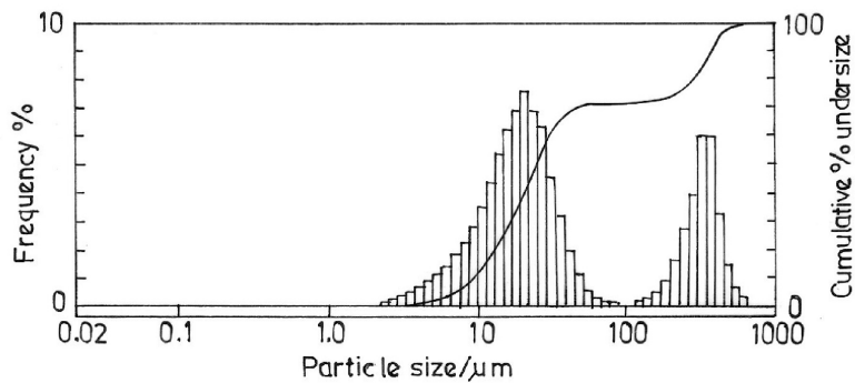
Fig. 5. Particle size pattern obtained for the NiAl 2 O 4 powder by combustion synthesis using glycine as a fuel
