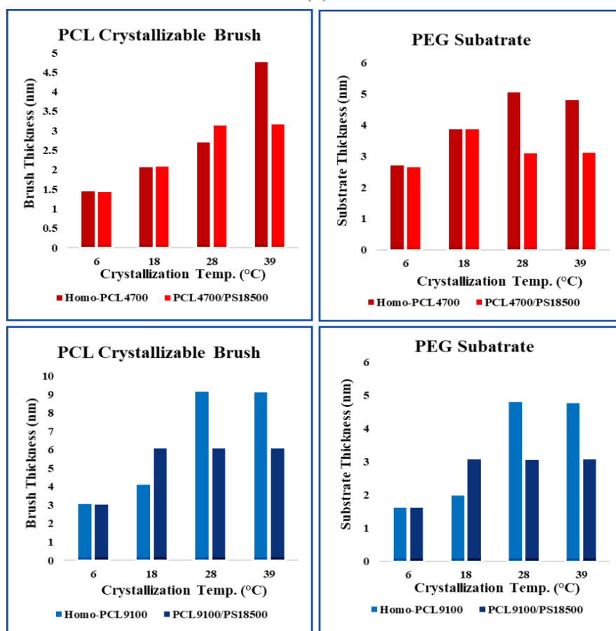
Fig. 3. AFM height images and the corresponding SAED patterns (a) as well as AFM height profiles (b) of PEG_{5000} - b - PS_{18500} / PEG_{5000} - b - PCL_{9100} single crystals grown at T_c = 6^\circ\text{C} (top) and T_c = 39^\circ\text{C} (bottom), in which the PCL brushes are amorphous and crystalline, respectively; the thickness trends of PCL brushes and PEG substrate via altering the crystallization temperature in PEG_{5000} - b -PCL and PEG_{5000} - b - PS_{18500} / PEG_{5000} - b -PCL single crystals (c).
