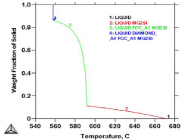
Fig.2. The solid fraction-temperature diagram achieved by Thermocalc.
