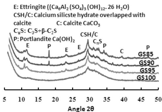
Fig. 7. X-ray patterns of HVS pastes after 28 days of hydration
