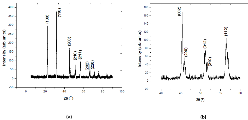
Fig. 11. Diffraction pattern of microwave sintered KNN ceramic, (a) Full scan of 2θ and (b) Selected part showing XRD patterns between 40° to 60° 2θ.
