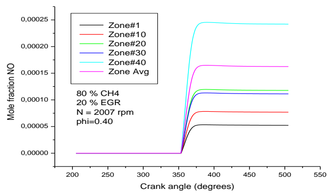
Fig11. Mole fraction of NO per CA histories (80 % CH4/ 20% EGR, phi = 0.40)
