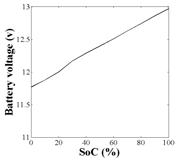
Fig5.: Open circuit voltage of battery [9]
