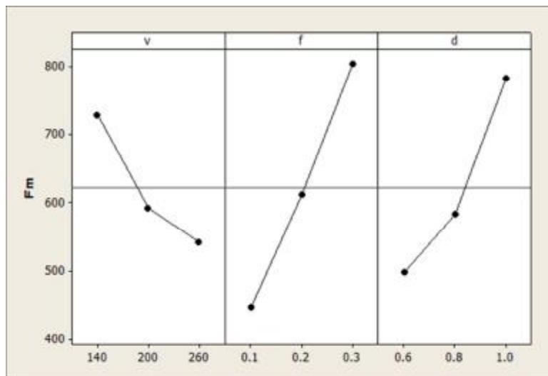
Fig3. Main effect plots for machining force (Fm)
