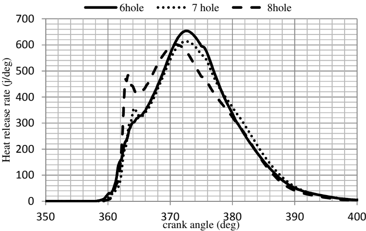
Fig8. Heat release rate in different cases
