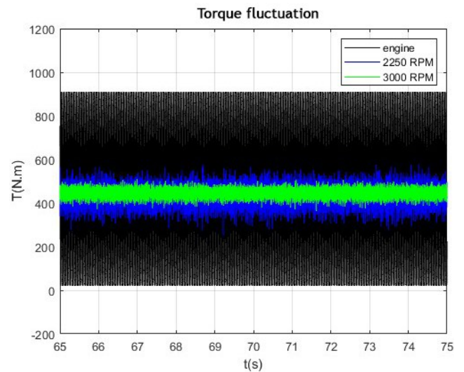
Figure 18: Engine and flywheel torque during loading
