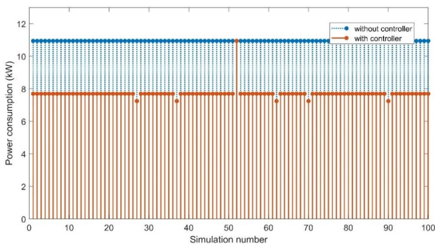
Figure 29: Maximum APU power consumption in 100 simulations
