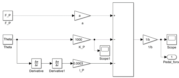
Figure 4: Pedal Model in Braking System
