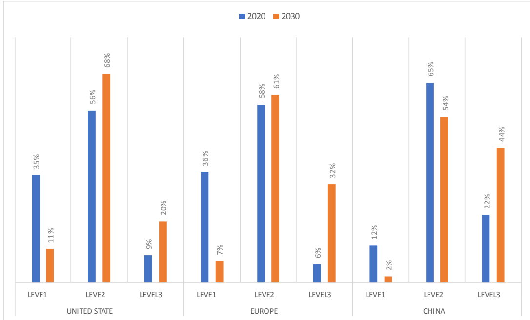
Figure 1: Energy demand by charging model [47]
