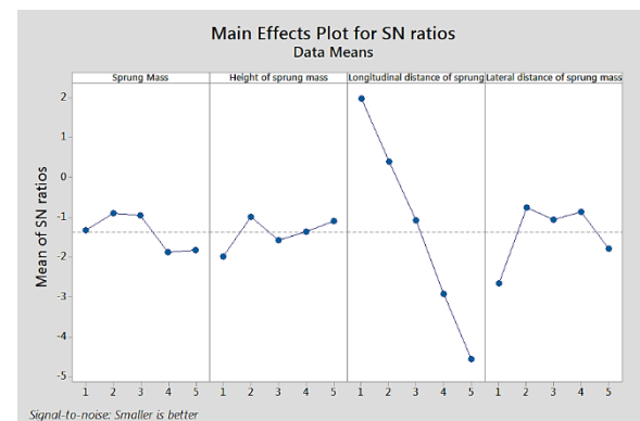
Figure45: Taguchi SNR plot for Sprung Mass properties
