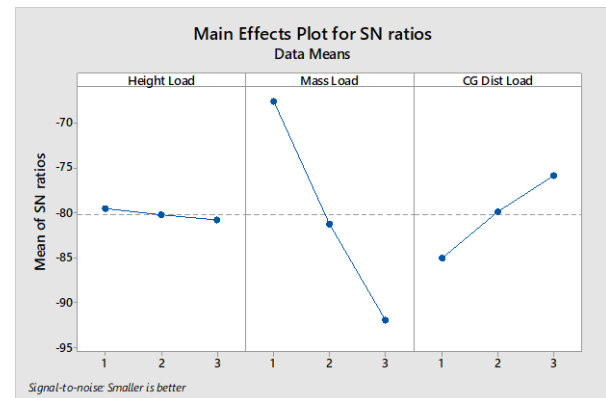
Figure22: First Step Taguchi for Load Factors
