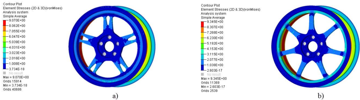
Figure 33: Von Mises stress of Tire Inflation pressure, a) Optimized Wheel A, b) Wheel in the market
