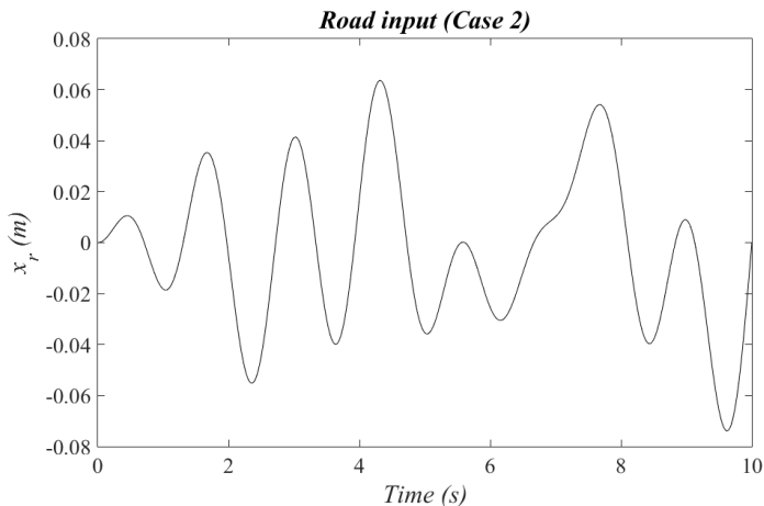
Fig4.Road input case 2 [12].
