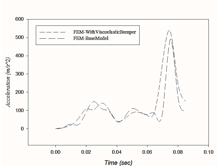
Fig22. Figure 22 Effects of the viscoelastic nature of the bumper material on time history of the acceleration of the occupant's body
