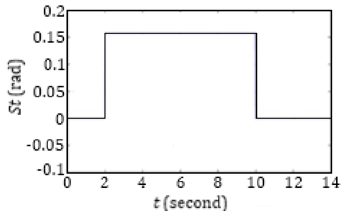
Figure 10: Steering wheels angle diagram in step steering maneuver
