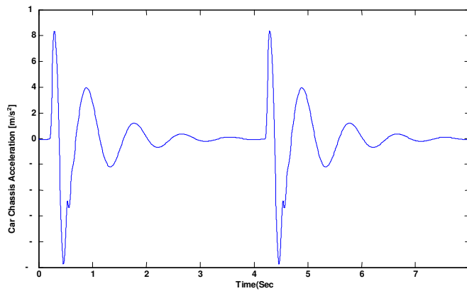
Fig11. The acceleration of the car chassis for isolated bumps
