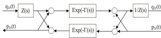
Fig3. Schematic of the two-port network used for pipeline model.
